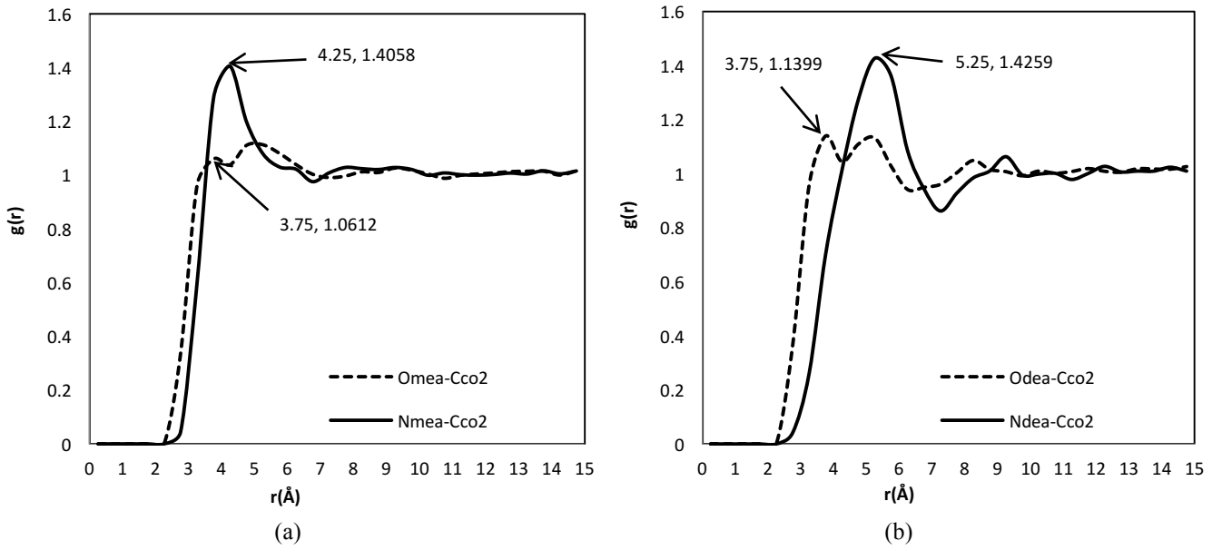
Figure 8: Intermolecular interaction of (a) MEA and (b) DEA solutions with CO 2
