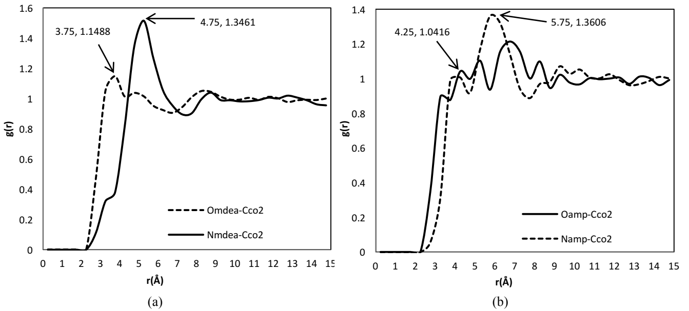
Figure 9: Intermolecular interaction of (a) MDEA (b) AMP solutions with CO 2
