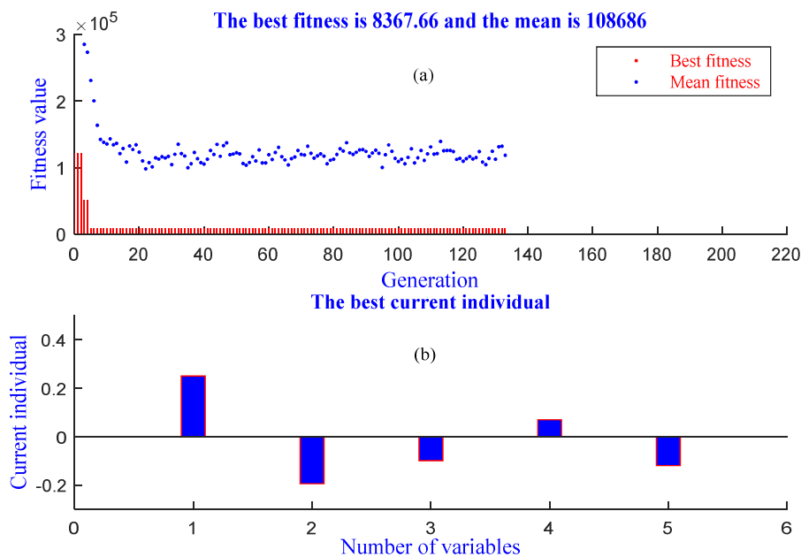
Figure 3. Using the GA approach to solve the ED problem (a) Best and mean fitness and (b) Best current genes Individual.
