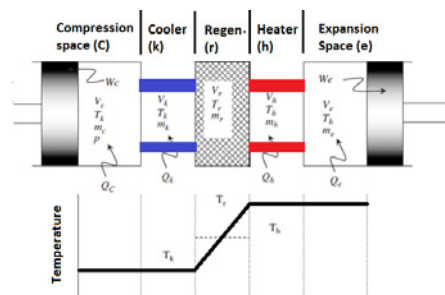
Fig. 1. Calculation model
