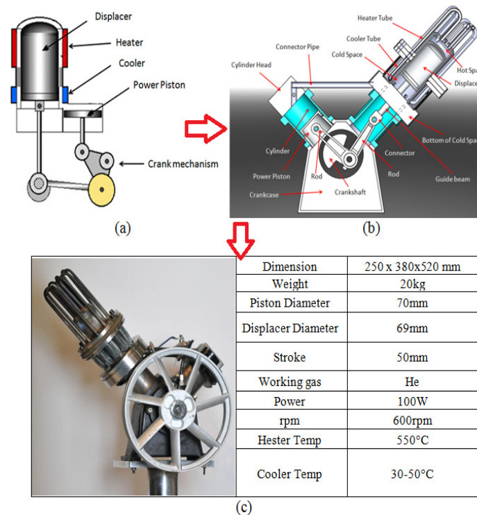
Fig. 2. (a) and (b) Schematic diagram of Stirling engine , (c) Real Stirling engine and its specifications
