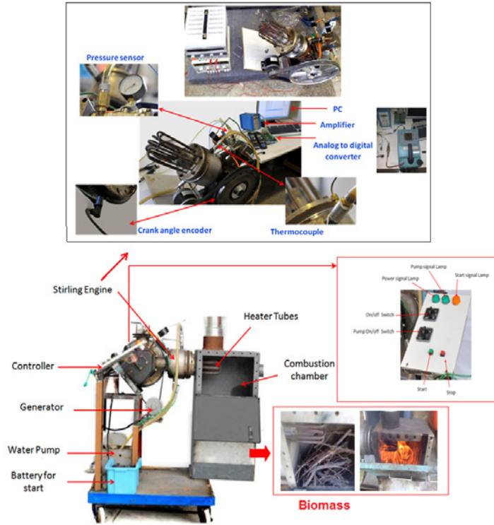
Fig. 3. Coupling of Stirling engine with micro combined heat and power (MCHP) system
