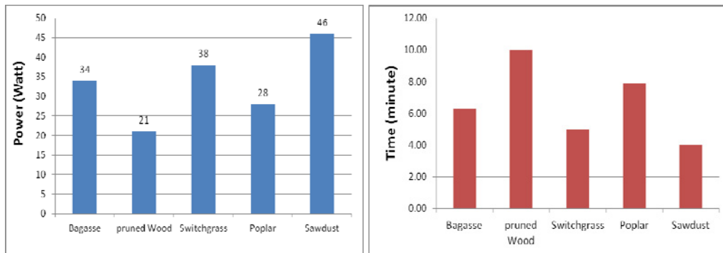
Fig. 7. Electrical power produced from burning of biomass and flammable agricultural wastes (biomass sources) (b) Ignition time of biomass sources
