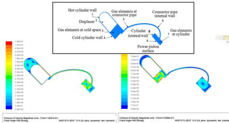
Fig. 4. CFD analysis of Stirling engine
