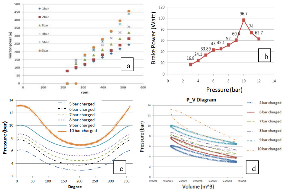
Fig. 6. (a) Friction power, (b) Brake power and (c) Indicated power (pressure) of tested stirling engine, (d) P-V diagram
