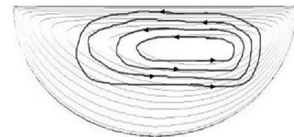
Fig 4. Particle positioning and path for Reynolds Number of 500
