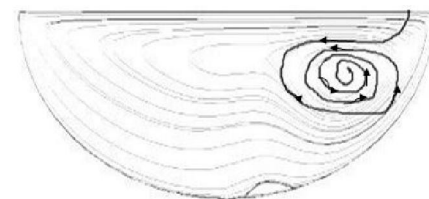
Fig 5. Particle positioning and path for Reynolds Number of 1500
