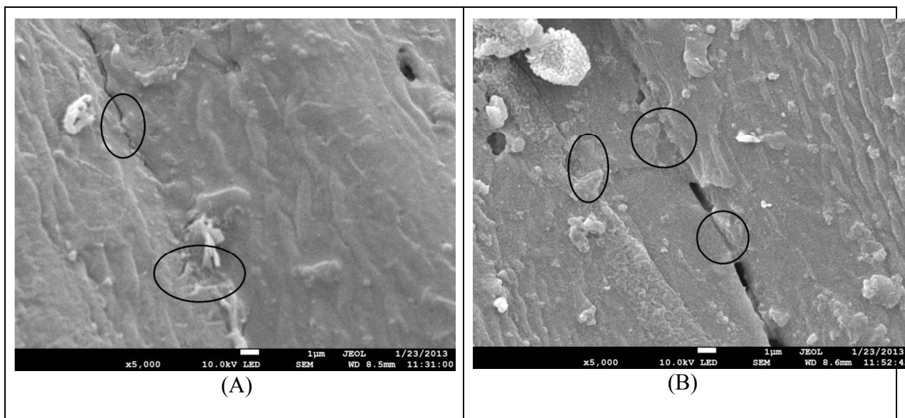
Figure 7: FE SEM of MDF boards at 5k magnification. (A) Prepared from UF 10% (B) Prepared from 3h treated fiber and Con-EHL 10%.
