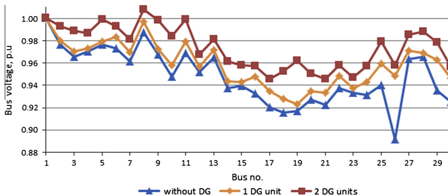
Fig. 12. Voltage profile for IEEE 30-bus with DG.
