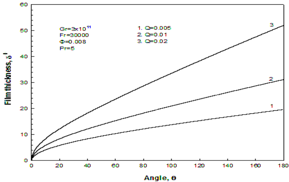
Figure 2. Variation of condensae film thickness around the periphery
