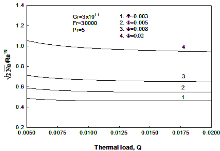
Figure 8. Effect of dimensionless heat flux on mean condensate Nusselt-Influence of interfacial shear
