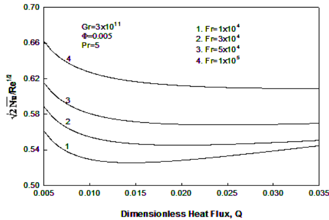
Figure 7. Effect of dimensionless heat flux on mean condensate Nusselt-Influence of Froude
