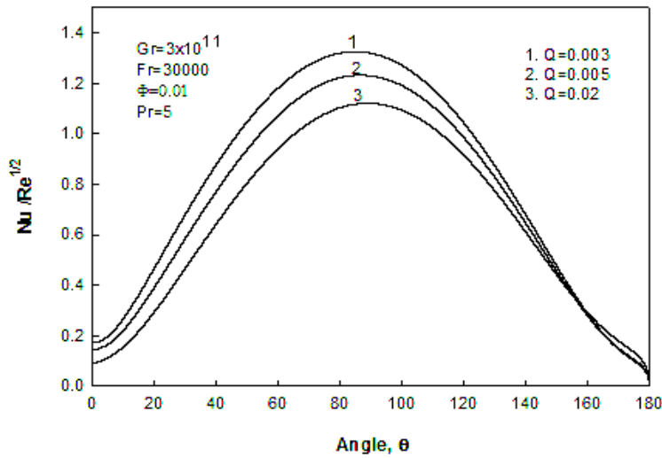
Figure 5. Variation of local Nusselt around the periphery-effect of Q
