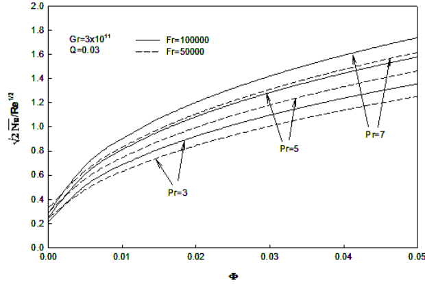
Figure 9. Effect of shear parameter on mean condensate Nusselt
