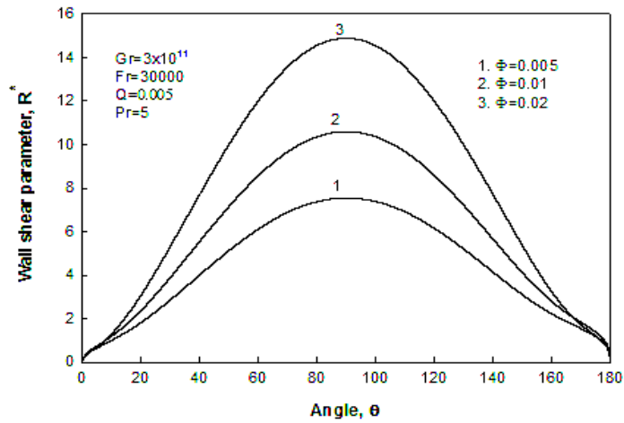
Figure 3. Variation of shear at the tube wall around the periphery- Effect of interfacial shear
