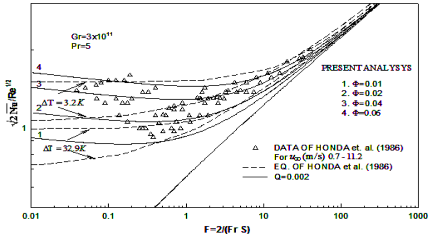
Figure 11. Comparison of present analysis with data of Honda et al. (1986)
