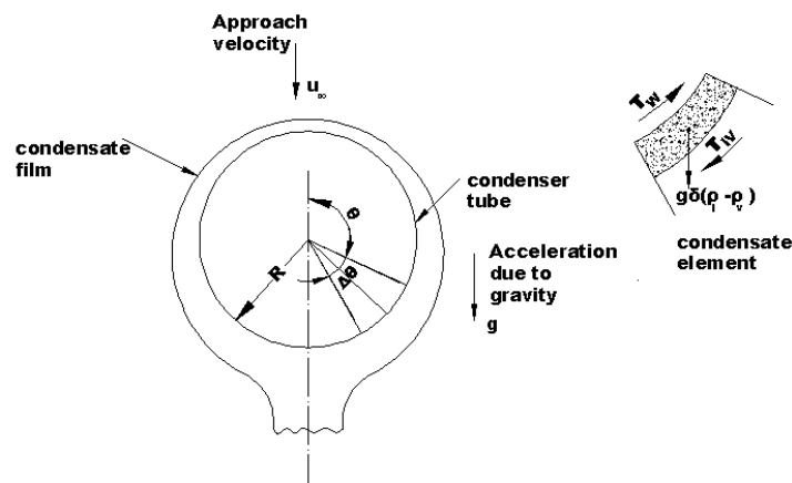
Figure 1. Physical configuration-flow model
