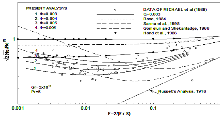
Figure 10. Comparison of present theory with experimental data of Michael et al. (1989) and Rose (1984)
