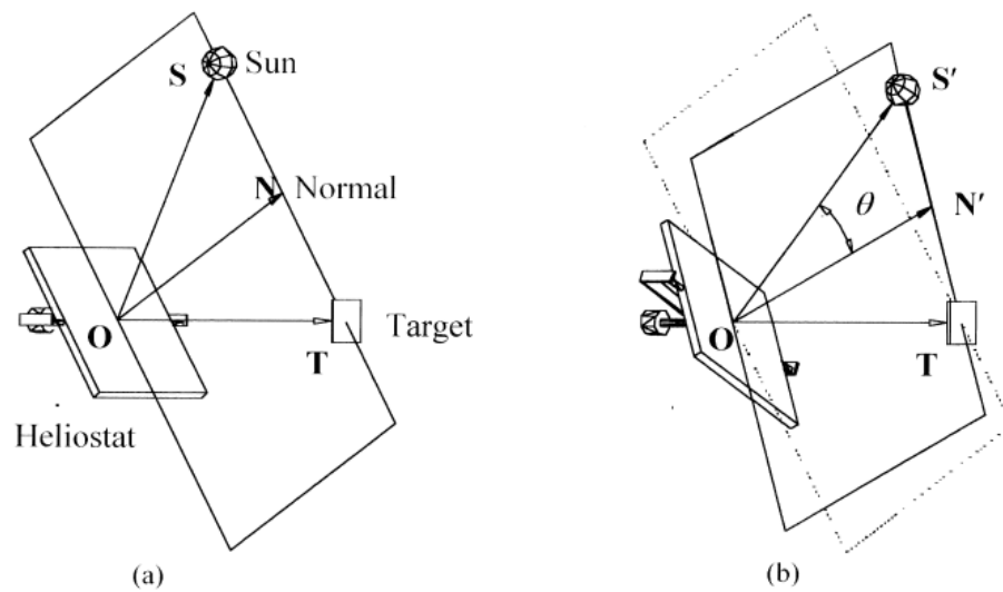
Figure 3.1: Rotation modes of rotation and elevation tracking technique
