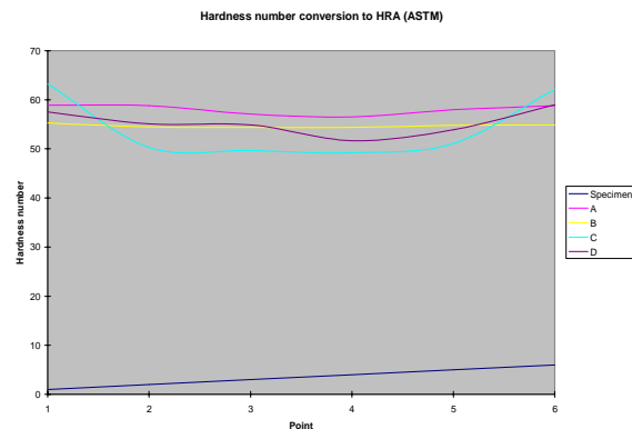
Figure 5: Hardness number conversion to HRA
