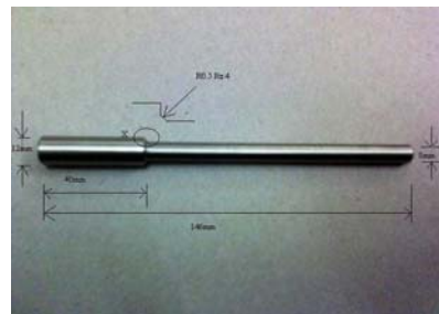
Figure 1: Standard size of fatigue specimen.
