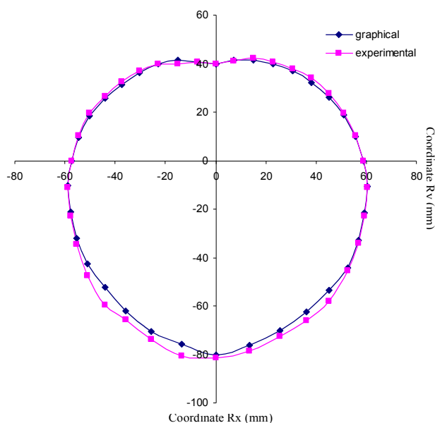
Figure 10. Comparison of cam profile between graphical and experimental methods
