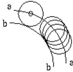
Figure 2. The trace point of the follower on a plate cam
