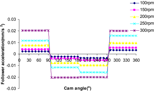
Figure 9. Follower acceleration diagram in 5 different speeds.
