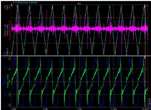
Figure 6. Graphs of output data of 100 rpm for one complete cycle
