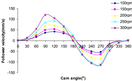
Figure 8. Follower velocity diagram in 5 different speeds
