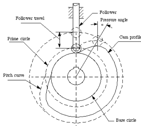
Figure 1. Cam Nomenclature [3]
