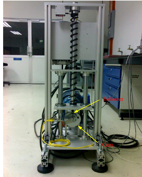
Figure 5. Cam mechanism analysis system
