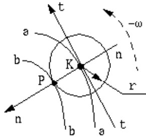
Figure 3. The tangent point, P, of a roller to the plate cam
