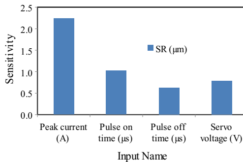
Fig. 7 Sensitivity analysis for surface roughness
