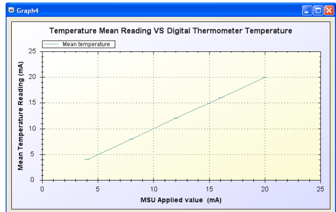
Figure 9. Calibration curve
