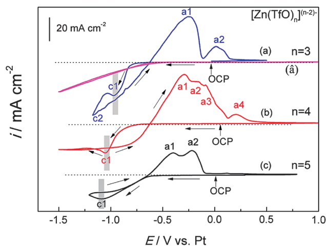
Fig. 5 The cyclic voltammograms of pure [\text{MIm}]\text{TfO} (â), of 0.2 M \text{Zn}(\text{TfO})_2/[\text{MIm}]\text{TfO} (a), of 0.2 M \text{Zn}(\text{TfO})_2/[\text{EMIm}]\text{TfO} (b) and of 0.2 M \text{Zn}(\text{TfO})_2/[\text{EMMIm}]\text{TfO} (c), respectively, recorded on gold at 120^\circ\text{C} . Scan rate: 10\text{ mV s}^{-1} .
