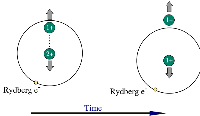
Figure 8.5: Frustrated triple ionization of an argon dimer.
