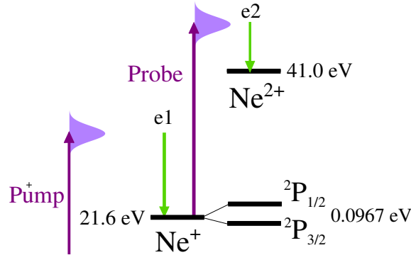
Figure 9.28: Energy level scheme illustrating the experiment on sequential TPDI of neon at \hbar\omega = 44 \text{ eV} . Explanations are given in the text.
