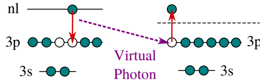
Figure 2.7: Illustration of the ICD of Eq. 2.68. The excited nl electron of the initial \text{Ar}^+(3p^{-2}nl) - \text{Ar} state fills a 3p^{-1} hole and the excess energy is transferred via a virtual photon (dashed purple arrow) to the neutral site of the dimer which is ionized.
