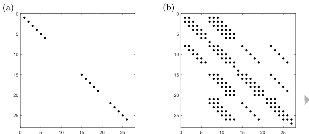
Figure 4: Plots to show the positions of the nonzero entries (black dots) in the mass matrix \mathbf{M} , panel (a), and the Jacobian matrix of \mathbf{f} , panel (b), for the finite difference scheme in the case N = 6 .
