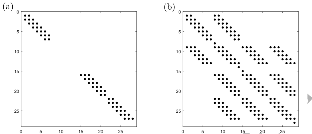
Figure 3: Plots to show the positions of the nonzero entries (black dots) in the mass matrix \mathbf{M} , panel (a), and the Jacobian matrix of \mathbf{f} , panel (b), for the finite element scheme in the case N = 6 .
