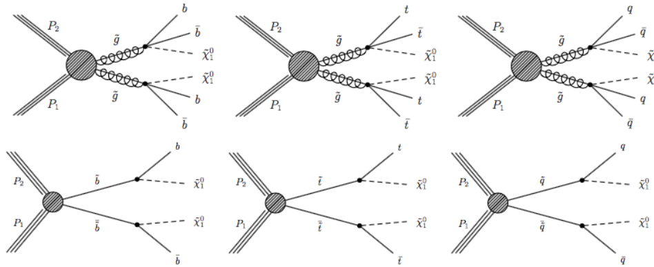
Fig. 2 The CMS collaboration, Khachatryan, V., et al., J. High Energ. Phys. (2016) 2016: 6, p. 20. doi:10.1007/JHEP10(2016)006 . Copyright: CERN / CMS under CC BY 4.0.
