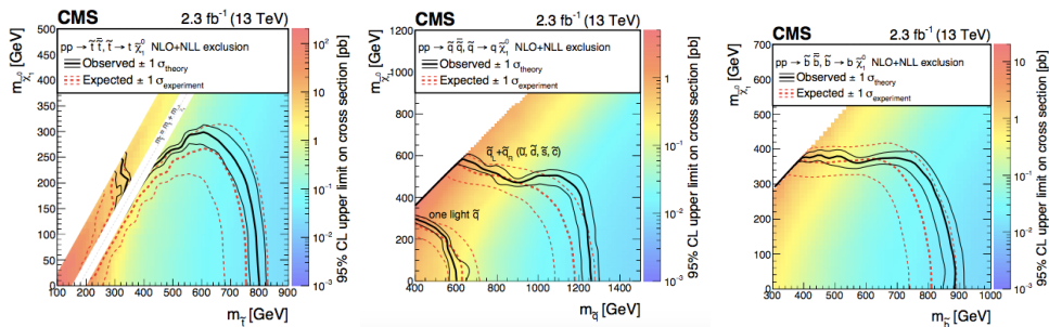
Fig. 4 The CMS collaboration, Khachatryan, V., et al., J. High Energy Phys. (2016) 2016: 6, p. 23. doi:10.1007/JHEP10(2016)006 . Copyright: CERN / CMS under CC BY 4.0.
