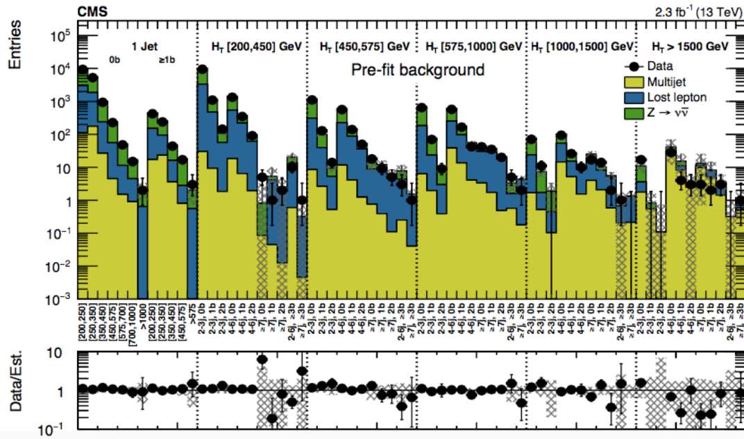
Fig. 3 The CMS collaboration, Khachatryan, V., et al., J. High Energy Phys. (2016) 2016: 6, p. 18. doi:10.1007/JHEP10(2016)006 . Copyright: CERN / CMS under CC BY 4.0.
