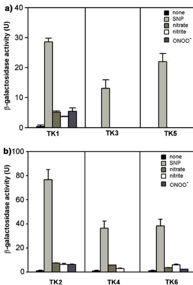
Fig. 2 Transcription of a P_{fhp} and b P_{fhpR} in PAO1 (TK1 and TK2), PA0779 mutant (TK3 and TK4) and PA3697 mutant (TK5 and TK6) under aerobic conditions. Cultivations were supplemented with sodium nitroprusside (SNP; 3 mM; light grey bars), nitrate ( \text{NO}_3^- ; 80 mM; middle grey bars), nitrite ( \text{NO}_2^- ; 20 mM; white bars) and peroxynitrite ( \text{ONOO}^- ; 1 mM; dark grey bars) 3.5 h after inoculation. Promoter activity was measured as \beta -galactosidase activity, which represents the promoter activity at 0.5 h after supplementation. Mean values and standard deviations of four separate cultivations are shown
