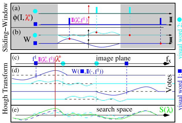
Fig. 3 (Color online) From Sliding-Window ( top ) to the Hough Transform ( bottom ). Shift-invariant 1D-example with four extracted features (c) quantised into two visual words (blue rectangle and cyan circle). Sliding-window reasoning ( top ): A single hypothesis \lambda^* is fixed (red). Its footprint (a) is a sum of Dirac pulses which are positioned according to the invariant \mathbb{I}(\lambda^*, f) = f - \lambda^* (depicted in (a, c) for f^1 ). This aligns the features to the object model. The inner product with the weight function (b) results in a sum of point evaluations (red dots). Features falling into the range where the weight function is zero (shaded) do not affect the score. Hough-Transform view ( bottom ): all features are considered simultaneously. Extracted features (c) cast voting patterns (d) which, summed up, result in the final hypothesis score (e). The voting patterns are transformed (e.g., mirrored and shifted) versions of the weights W . Their intersections with the red line corresponds to the red dots in the sliding-window setting (b). The solid green curve (e) shows the overall hypothesis score and one can identify \lambda^* as a local maximum. The alternation of greedy search and feature suppression (c.f. Sect. 2.5) implements a matching pursuit like algorithm to recover the sparse semantic description (i.e., “a car at position \lambda^* ”) from the blurry semantic reconstruction (e)
