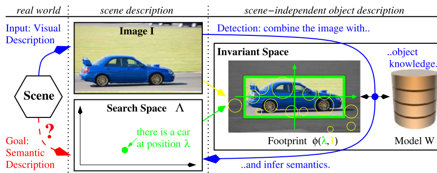
Fig. 1 (Color online) High-level illustration of PRISM’s main concepts. The goal of object detection is to recover a semantic description of a scene (e.g. “a car at position \lambda ”) while we only have access to a visual description, i.e. , the image pixels. Both visual and semantic description are scene-dependent and cannot be accessed during training (as they do not exist then). Our object footprint couples them and allows for computing a scene-independent object description for each object hypothesis. This footprint compensates for (geometric)
