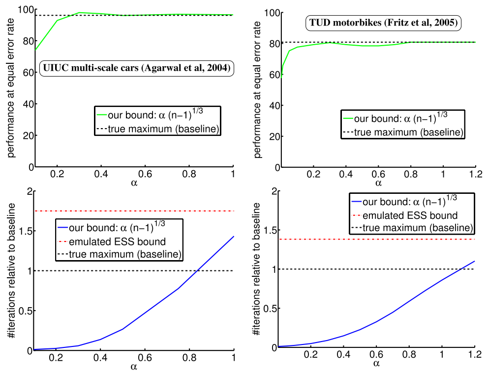
Fig. 12 (Color online) Evaluation of the probabilistic bounds in terms of performance at equal error rate ( top ), and number of iterations relative to the baseline ( bottom ). As baseline we consider a system which has access to the true maximum in (10). The results are shown for UIUC multi-scale cars ( left ) and TUD motorbikes dataset ( right ). From the top plots we see that our probabilistic bound performs well for values \alpha > 0.2 and breaks down for smaller values. For a safe choice of \alpha = 0.3 , the number of iterations is just about 6% ( left ) and 8% ( right ) compared to the baseline system. In comparison, ESS's uses a true bound which converges slower than the baseline by a factor of about 1.7 and 1.5, respectively
