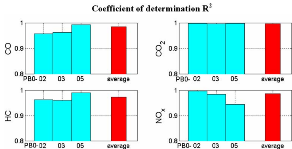
Fig. 5 Coefficient of determination ( R^2 ) for the pre-Euro-1 gasoline vehicles (blue) and for the group of pre-Euro-1 gasoline cars (red)
