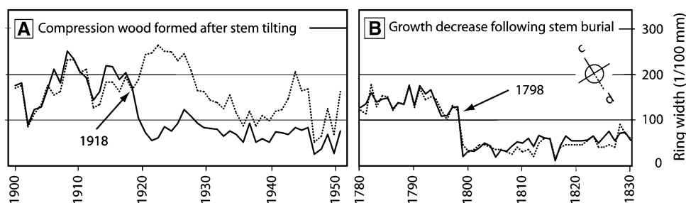
Fig. 5 Examples of growth disturbances inferred by debris-flow activity: a after tilting in AD 1918, this P. abies tree initiated the formation of compression wood cells on the tilted side of its trunk (i.e. core c ) so as to regain a vertical position. Most of the tree's energy is
