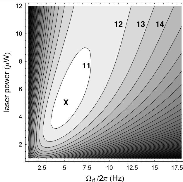
Fig. 7 Plot of \delta B_{NEM} as a function of the amplitude \Omega_{rf} of the rotating field and of the laser power P_L . The contours represent the lines of constant NEM, spaced by 1 \text{ fT}/\sqrt{\text{Hz}} , with selected numerical values indicated. The cross refers to the minimal NEM value, which, for the cell represented here has a value of 10.5 \text{ fT}/\sqrt{\text{Hz}}
