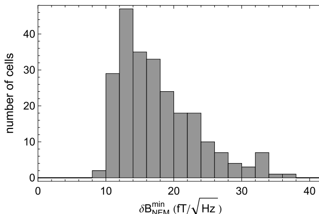
Fig. 8 Histogram of the minimal NEM values, \delta B_{NEM}^{\min} , of 241 cells, which represent 94% of the cells produced to date
