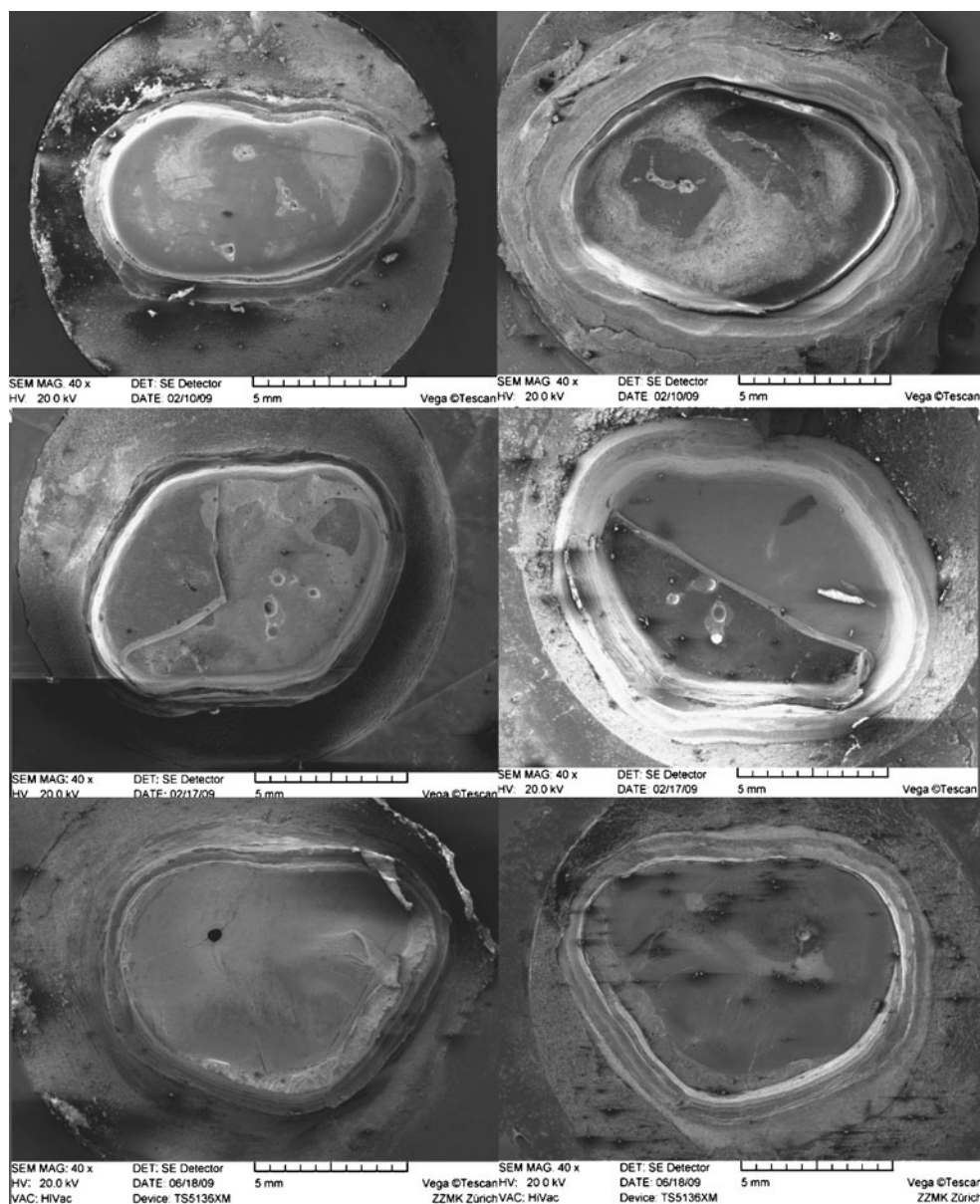
Fig. 6 SEM picture: failure type 1—failure in the interface dentin and cement; type 2—mixed failure; and type 4—failure in the coronel or root
