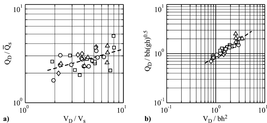
Fig. 8a, b. Maximum water displacement rate. a Q_D/Q_s vs. V_D/V_s with dashed curve, linear regression ( r^2=0.30 ) and open diamond, 2 < F \leq 2.5 ; open circle, 2.5 < F \leq 3 ; open square, 3 < F \leq 4 ; open triangle, 4 < F < 5 ; b Q_D/(bh(gh)^{0.5}) vs. V_D/(bh^2) with Eq. (10) and symbols as in a.
