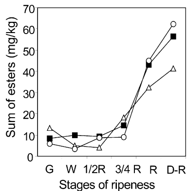
Fig. 4 Sum of volatile esters in Carezza ( black square ), Darselect ( white triangle ) and Marmolada ( white circle ) strawberries at different stages of ripeness. Stages of ripeness: G green, W white, 1/2 R half-red, 3/4 R three-quarters-red, R red-mature, D-R dark-red. Values are means of three replications
