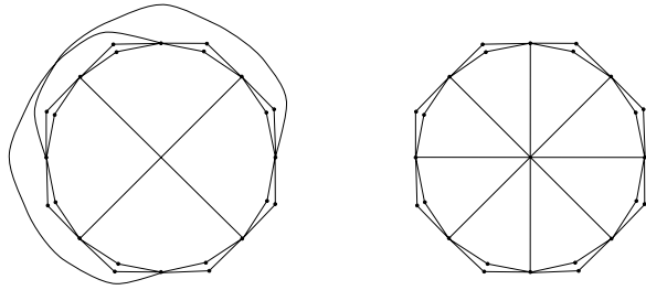
Fig. 1 CR(G) = 2, CR^*(G) = 1
