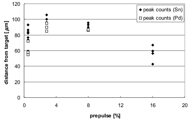
FIGURE 5 Distance of the 11.9-nm Sn X-ray laser emission zone from the target as a function of prepulse amplitude. Results for the 14.7-nm Pd X-ray laser from [14] are included for comparison
