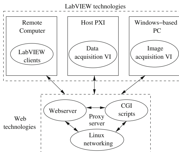
Fig. 3 Software architecture
