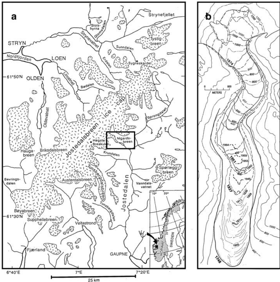
Fig. 2 a Map showing the Jostedal ice cap with its main branches. b The tongue of the Nigardsbreen Glacier and its foreland with dates of the formation of some of the moraines (Østrem et al. 1976). Contour lines are indicated for the years 1937 (dashed lines), 1951 (solid lines) and 1974 (grey lines)
