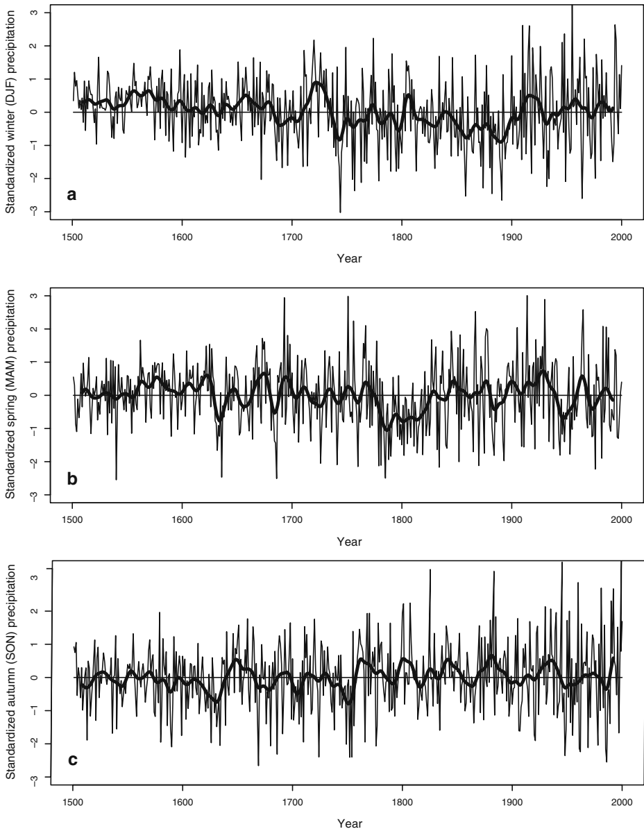
Fig. 7 Standardized precipitation values for the 1500–2000 period ( solid lines ) at the grid point 8.25° E/ 46.75° N (Lower Grindelwald Glacier; after Pauling et al. 2006): a winter (DJF) precipitation, b spring (MAM) precipitation, c autumn (SON) precipitation. Also shown are the 20-year low-pass filtered time series of the precipitation model inputs ( thick lines ). The time series are z-standardized relative to the 1535–1983 mean and standard deviation
