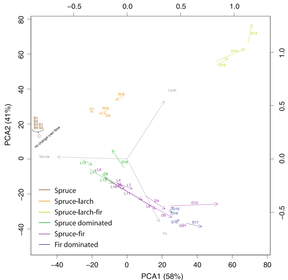
Fig. 7 Principal components analysis (PCA) of overstory tree species composition (Importance Value) for first and last inventory, showing the temporal dynamics of species composition. Note that the time elapsed for the trajectories shown varies between permanent plots. Colors according to groups from cluster analysis. Vectors for major tree species are marked in grey
