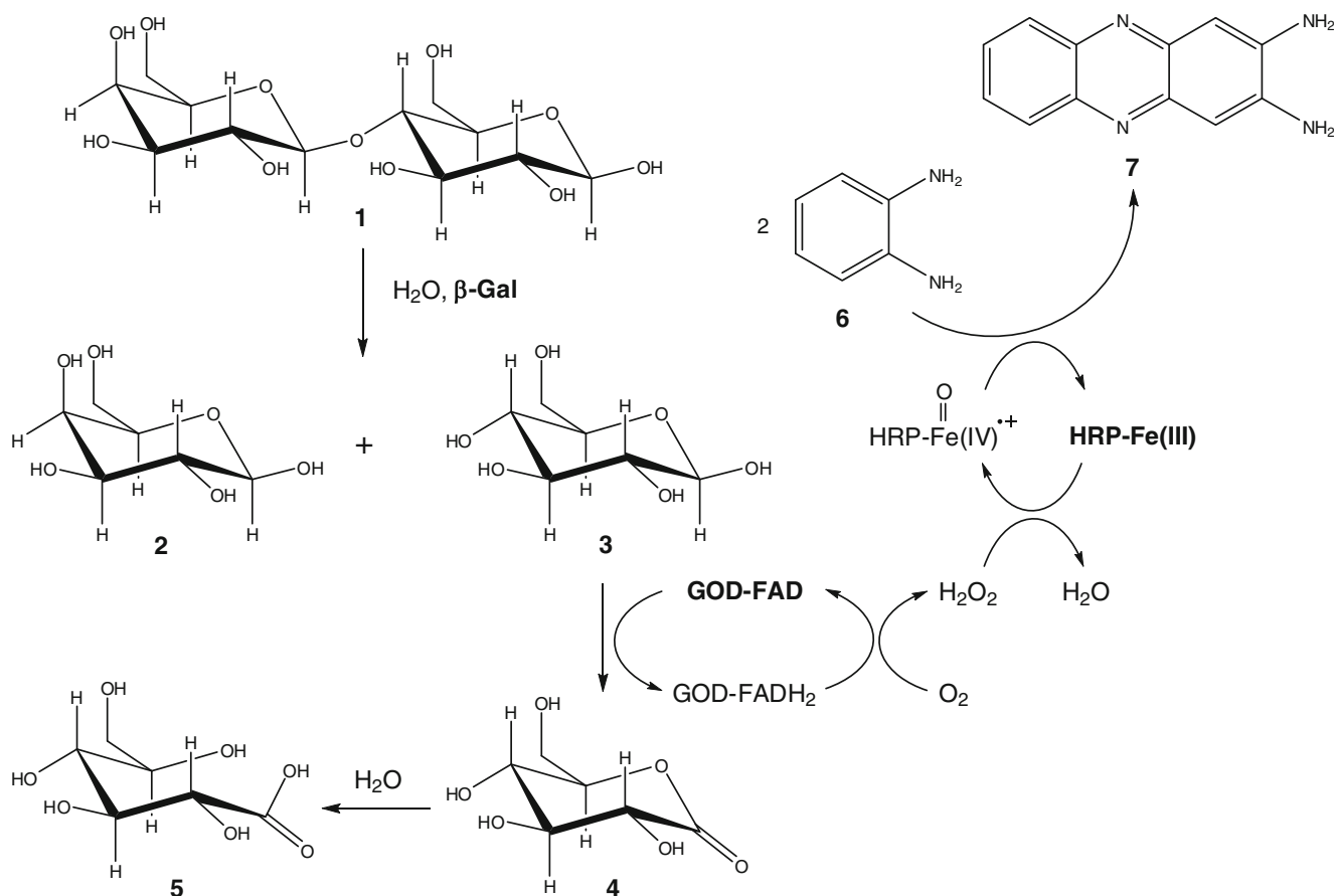
Scheme 1 Outline of the enzymatic cascade reaction system used for the quantification of lactose. The hydrolysis of lactose (1) into D-galactose (2) and D-glucose (3)—partially via the intermediate formation of allolactose—is catalyzed by \beta -Gal [13]. The \beta -form of D-glucose (3) is oxidized by the FAD-dependent GOD to glucono- \delta -lactone (4) and H 2 O 2 . During this reaction step, the coenzyme FAD is reduced to FADH 2 , which, in the presence of O 2 , is reoxidized to
