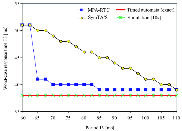
Fig. 11 Analysis results for the WCRT of T3 in benchmark 1
