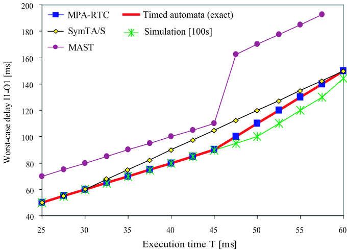
Fig. 18 Analysis results for the worst case delay II–OI in benchmark 5
