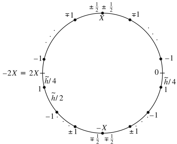
Fig. 1 Nodes and weights for the quadrature rules in Appendix. When two signs appear, the top one is for N even, the other for N odd
