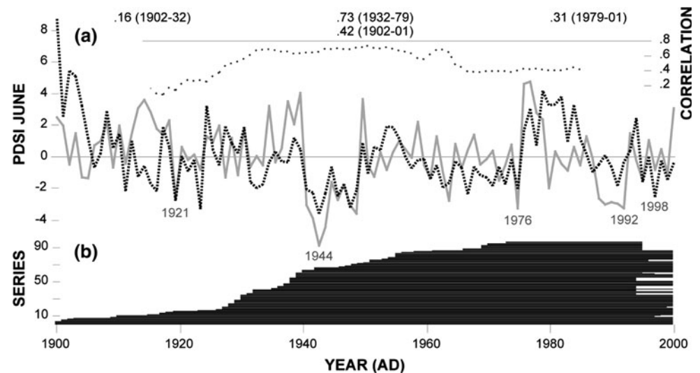
Fig. 3 a Comparison of the colline chronology ( black dashed ) and June scPDSI ( gray ). The TRW proxy was scaled (i.e., their variance and mean adjusted) to the climatic target (1901–2002), black dots indicate their 31-year moving correlations and b TRW sample replication is indicated
