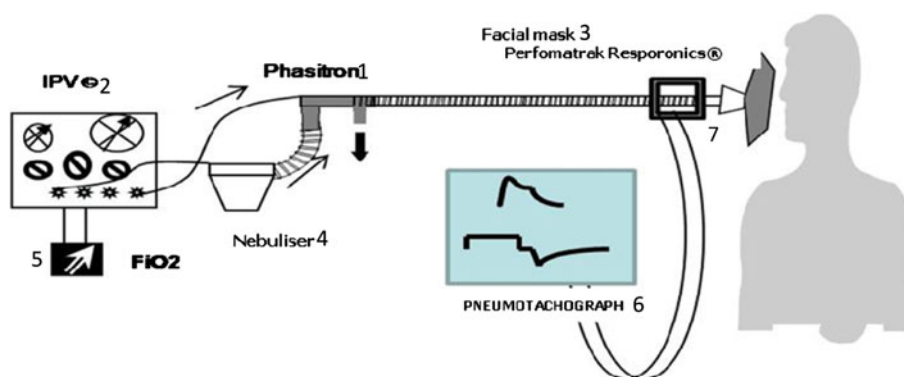
Fig. 1 Schematic representation of the circuit. Intrapulmonary percussive ventilation (IPV) provides a pulsatile flow; the Phasitron ® (1) in the IPV uses a sliding flow based on the venturi effect. Gas from the nebuliser is dragged through the Phasitron ® . The circuit is a single line connected to the IPV device (2). The face mask (3) was adjusted to the patient. Humidification was provided by the nebuliser (4). Only two parameters were set, pressurisation
