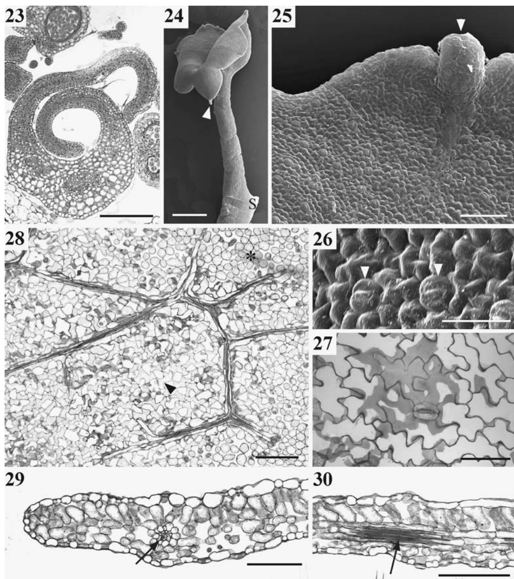
Figs. 23–30. Gunnera herteri (cult. BG Stockholm). Developmental and anatomical aspects of foliage leaves. 23. Young foliage leaf with involute blade vernation. Scale bar = 200 \mu\text{m} . 24. Oblique abaxial view of young seedling leaf with palmately lobed blade on elongate petiole. Arrowhead points to marginal tooth with hydathode. Note presence of sheath-lobe (S) at leaf base. Scale bar = 1 mm. 25. Overview of upper (“adaxial”) epidermis near blade margin. Note marginal hydathode (arrowhead). Scale bar = 100 \mu\text{m} . 26. Close-up of upper epidermis with stomates (arrowheads). Scale bar = 40 \mu\text{m} . 27. Another portion of upper blade epidermis, seen as surface view. Note presence of stomate surrounded by epidermal cells with wavy outlines (anomocytic type). Scale bar = 100 \mu\text{m} . 28. Paradermal section of blade portion, showing network of tiny vascular bundles, palisade parenchyma (asterisk) and spongy parenchyma (arrowhead). Scale bar = 200 \mu\text{m} . 29, 30. Marginal and more proximal cross-section of leaf-blade, respectively. The chlorenchyma consists of single-layered palisade parenchyma and up to three layers of spongy parenchyma. Arrows point to vascular bundles in transverse and longitudinal sections. Scale bars = 200 \mu\text{m}
