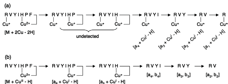
Scheme 1. Fragmentation of angiotensin III induced by copper ions. Experiments ran with (a) a Cu electrode and (b) a Pt electrode in presence of \text{CuCl}_2 .
