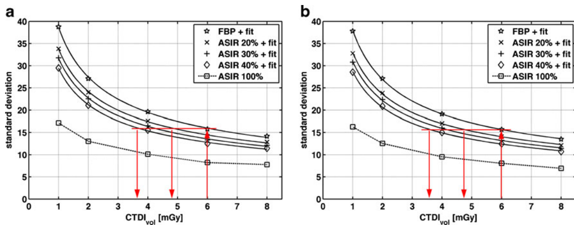
Fig. 7 SD as a function of CTDI_{vol} for different ASIR percentages and two tube voltages: 80 kVp (a) and 100 kVp (b). Acquisitions were performed with the paediatric protocol on the paediatric phantom. A SD of 15.5 HU is measured at 6 mGy with the FBP method while the same
