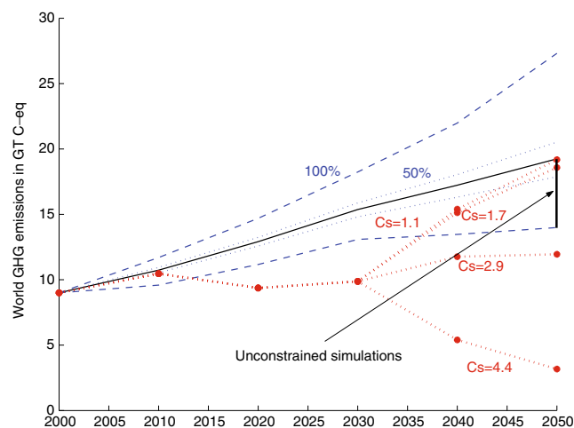
Fig. 13 Uncertainty in emissions projections
