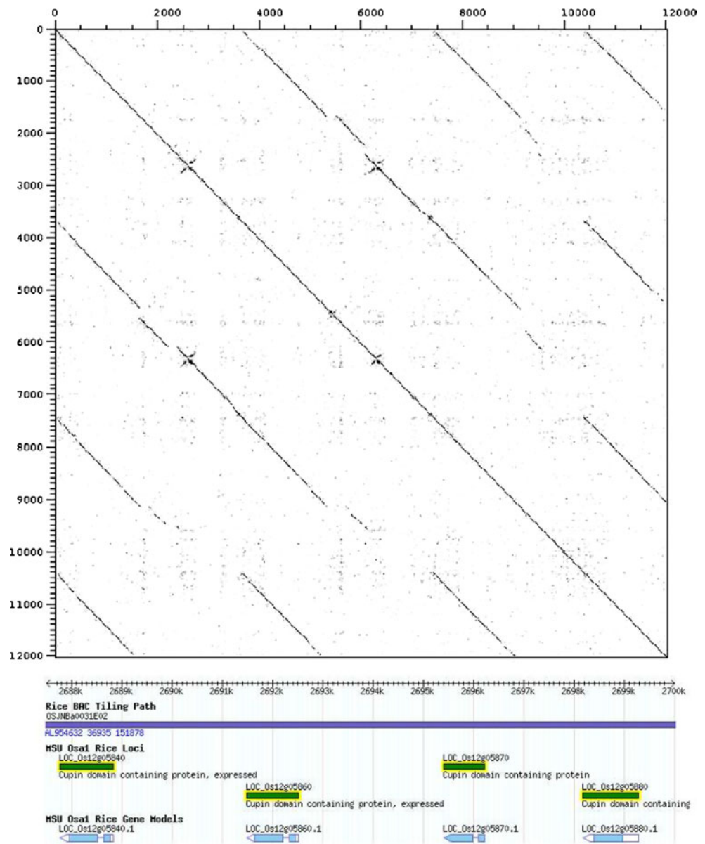
Fig. 4 A self dot-plot of a 12 kb sequence on rice chromosome 12 (2, 687, 500–2, 699, 500 bp) that contains four GLP genes. Located below the figure is the corresponding sequence annotation from the MSU (formerly TIGR) rice genome annotation database (Ouyang et al. 2007). The four GLP genes are coloured in green and highlighted in yellow and the red bars indicate repeats from the Oryza repeat database (Ouyang and Buell 2004)
