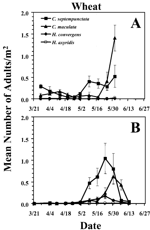
Figure 5. Mean ( \pm SEM) numbers of adult coccinellids per m 2 in wheat fields in 1995 (A) and 1996 (B). Sampling was initiated during tillering stage and ended near harvest.
