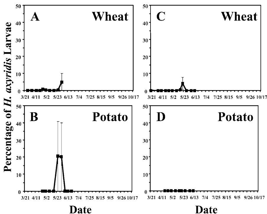
Figure 4. Mean ( \pm SEM) percentage of the overall predaceous coccinellid larval population that consisted of H. axyridis in wheat and potato in 1995 (A and B, respectively) and in 1996 (C and D, respectively).
