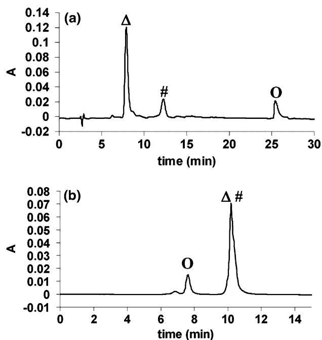
Fig. 7 High-performance liquid chromatography (HPLC) traces of 5 in BSA solution monitored at 360 nm after 24 h. a RP-C18 column for the analysis of B 12 compounds, starting material 5 (triangle) decomposition product free B 12 (hash) and cobalamin bound to BSA (circle). b Size-exclusion HPLC column, all cobalamins bound to BSA proteins (circle), and free cobalamins (triangle, hash)
