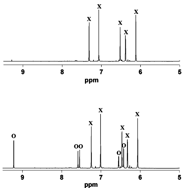
Fig. 2 ^1\text{H} NMR (500 MHz, \text{CD}_3\text{OD} , 27 °C) spectrum of pure [\{\text{Co}\}-\text{CN}-\{\text{trans-PtCl}(\text{NH}_3)_2\}]^+ ( 5 ) (top) and of a mixture of 5 base-on (X) and base-off (O) forms (bottom). For ease of comparison, only the downfield region from 5 to 9.5 ppm is shown here
