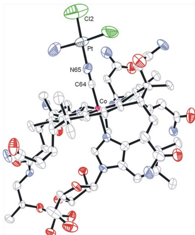
Fig. 4 ORTEP presentation of [\{\text{Co}\}\text{-CN}\{-\text{cis-PtCl}_2(\text{NH}_3)\}] ( 7 ), selected bond lengths (angstrom) and angles (degree): Co–C64 1.885(10), C64–N65 1.151(13), N65–Pt 1.940(10), Cl2–Pt 2.258(8), N65–C64–Co 178.2(10), C64–N65–Pt 174.5(9). Solvent molecules and hydrogen atoms were omitted for clarity
