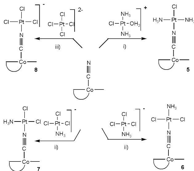
Scheme 1 Reagents and conditions for the preparation of conjugates [\{\text{Co}\}-\text{CN}-\{\text{Pt}\}] : i with trans -[PtCl(NH 3 ) 2 (H 2 O)] + → 5 , MeOH, 17 h at 45 °C, 77%; ii with [PtCl 3 (NH 3 )] – , MeOH, 18 h at 45 °C, 25% → 6 , 50% → 7 ; iii with [PtCl 4 ] 2– , MeOH, 10 days at room temperature, 35% → 8
