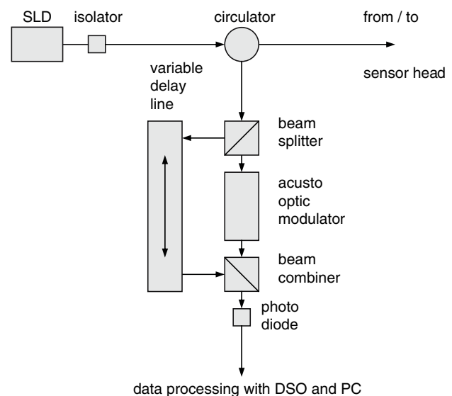
Fig. 2 Schematic setup of optical components in the interferometer unit, which also includes the light source
