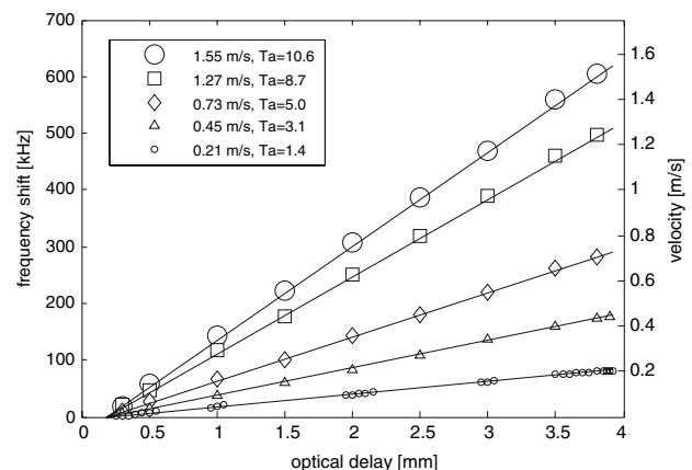
Fig. 6 SR-LDV measured Taylor-Couette flow profiles at different surface velocities. The marker size scales with standard deviation
