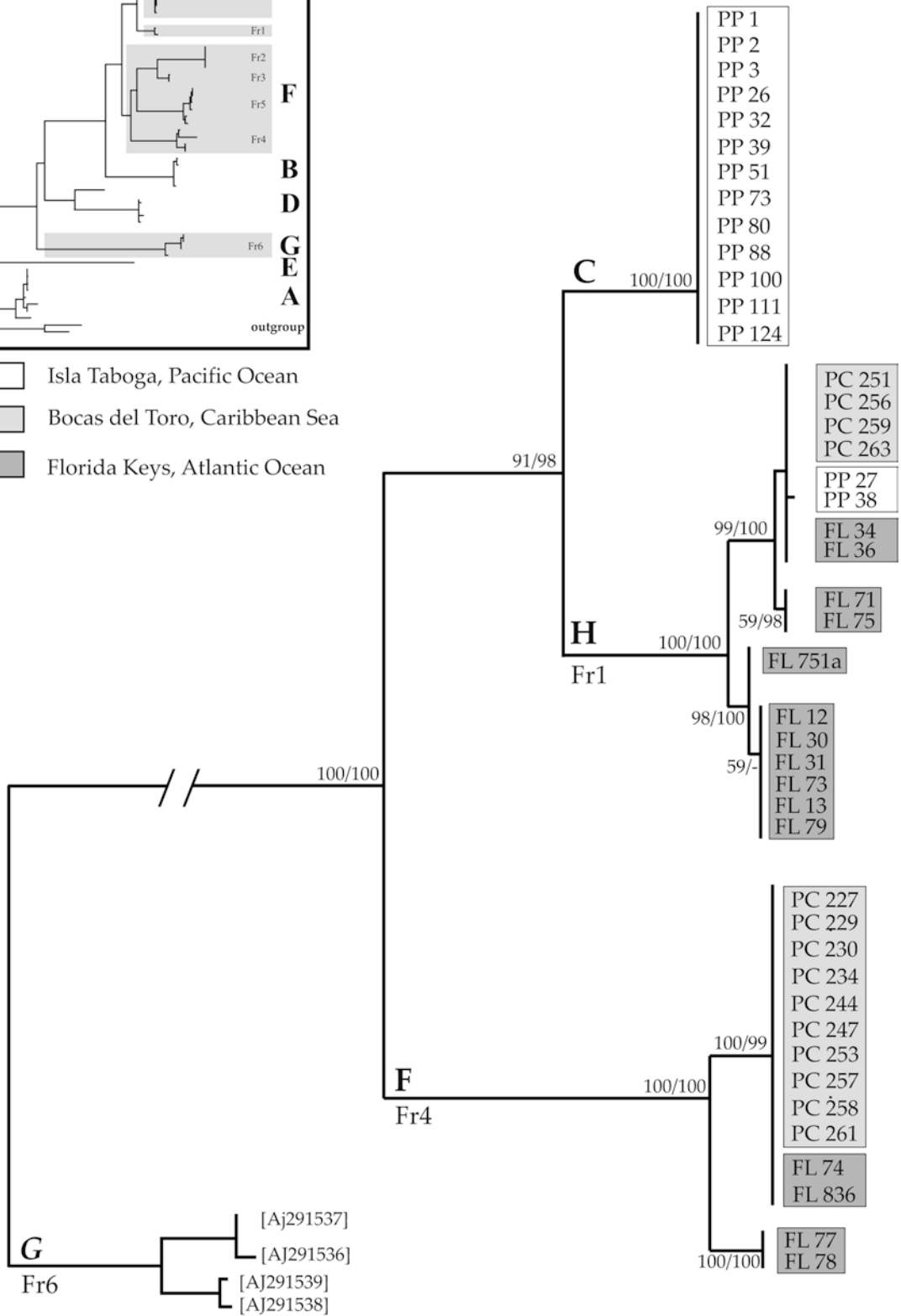
b 0.1 substitutions per site
