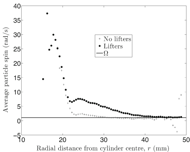
Fig. 8 Spin profiles for systems simulated with and without lifters for a fill level of 26%. The particles are 3 mm spheres and the cylinder has a diameter of 100 mm, a length of 152 mm and is rotated at 10 rpm
