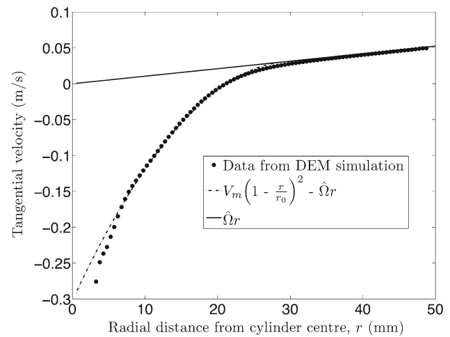
Fig. 4 Points tangential velocity profile for 19,380, 3 mm particles in a cylinder of diameter 100 mm and length 152 mm. The cylinder is rotated at 10rpm. Lines (1) with \hat{\Omega} = 10 \text{ rpm} , r_0 = 29 \text{ mm} and V_m = 0.302 \text{ m/s}
