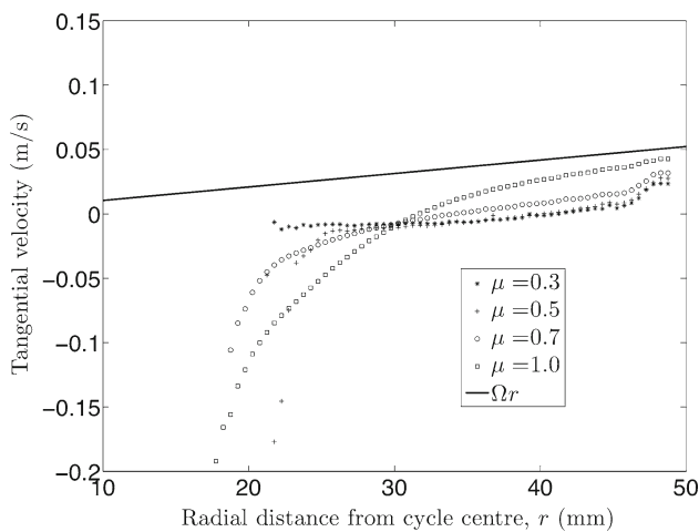
Fig. 5 Tangential velocity profiles for a range of coefficients of friction for f = 26\% . The particles are 3 mm spheres and the cylinder has a diameter of 100 mm, a length of 152 mm and is rotated at 10 rpm
