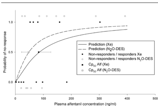
FIGURE 1 The predicted probability of no-response to skin incision ( C_{p50} ) is plotted in relation to the measured plasma alfentanil concentration. Responders and non-responders of the xenon group are represented by filled circles and those of the nitrous oxide ( N_2O )-desflurane group by open circles. The filled and open squares represent the C_{p50} of alfentanil in the xenon and the N_2O /desflurane group respectively (error bars = standard error of the estimate).
