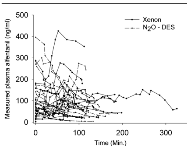
FIGURE 2 The measured plasma alfentanil concentrations between skin incision and closure are plotted for each subject. Solid lines with filled circles = xenon patients, dashed lines with triangles = nitrous oxide ( N_2O )/desflurane patients.
