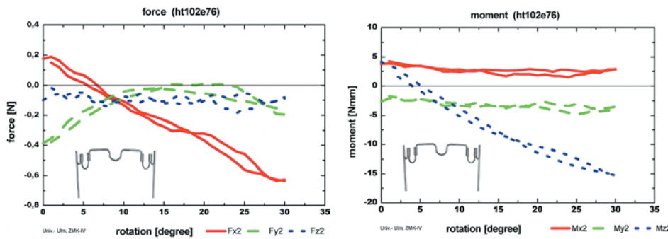
Figures 15a and 15b. Nickel-titanium/stainless steel transpalatal arch (Forestadent®), Compound palatal arch®, with rotation. Representation of forces and moments (a: forces, b: moments).
