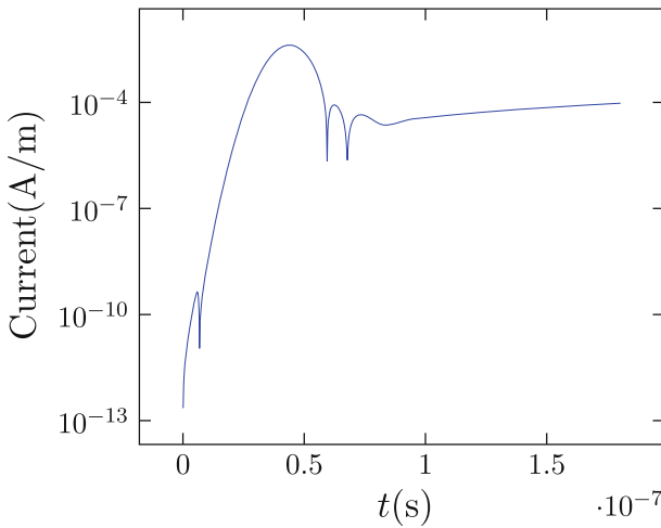
Fig. 2 Magnitude of the current at a point on the perfectly conducting sphere induced by an incident wave with center frequency f_0 = 0
