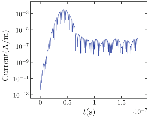
Fig. 1 Magnitude of the current at a point on the perfectly conducting sphere induced by an incident wave with center frequency f_0 = 200 MHz
