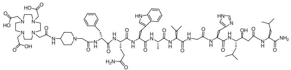
Fig. 1 Structure of unlabelled peptide chelator conjugate RM2
