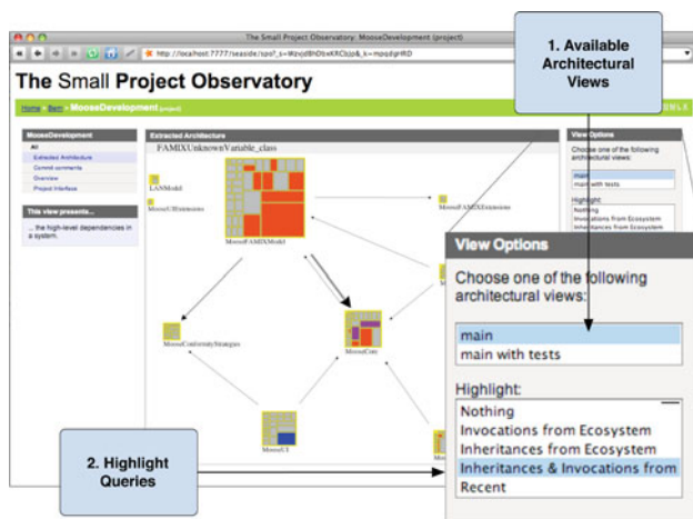
Fig. 6 Visualizing in SPO an architectural view that was generated in Softwareonaut
