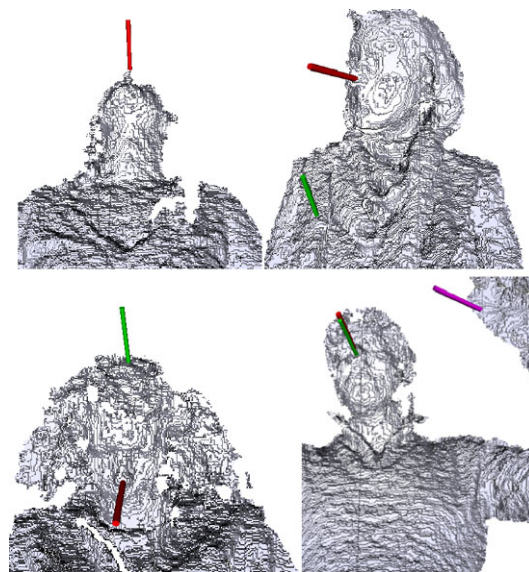
Fig. 22 Some typical failure cases of the algorithm, showing a missed detection and two false positives. The estimated head pose is shown in green , the ground truth is in red . The magenta cylinder indicates a (wrong) second detection (Color figure online)
